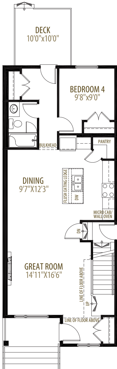
Main Floor 930 sq ft
