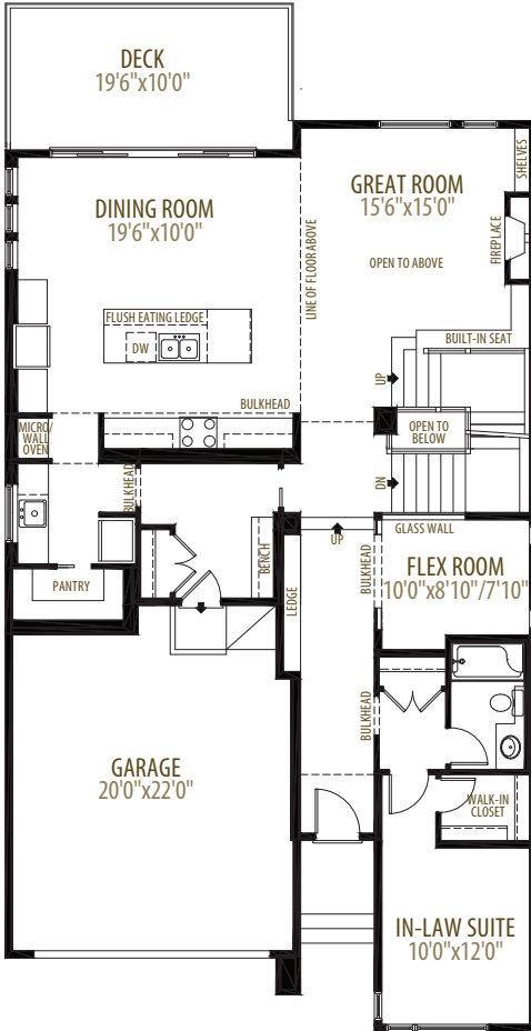
Main Floor 1,569 sq ft
