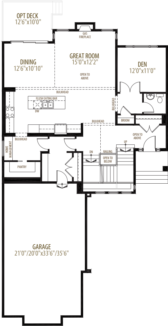
Main Floor 1,409 sq ft
