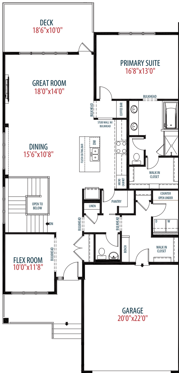
Main Floor 1,681 sq ft
