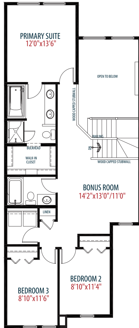
Upper Floor 1,038 sq ft
