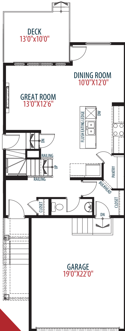
Main Floor 764 sq ft
