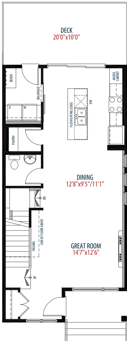
Main Floor 770 sq ft
