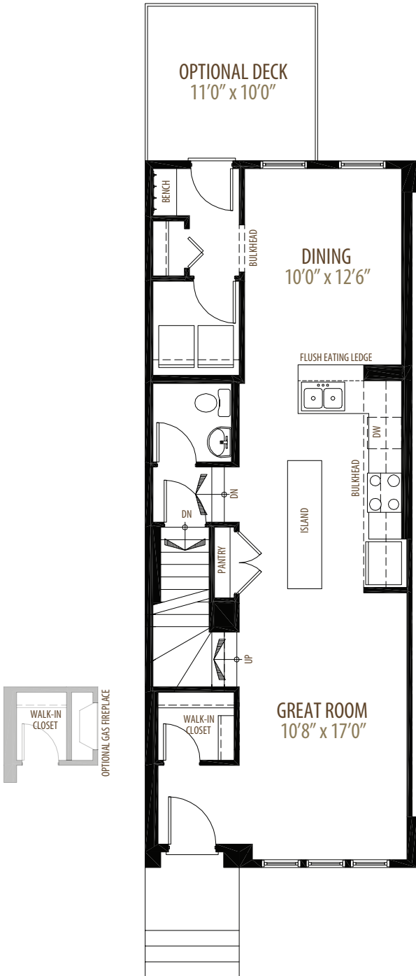
Main Floor 759 sq ft
